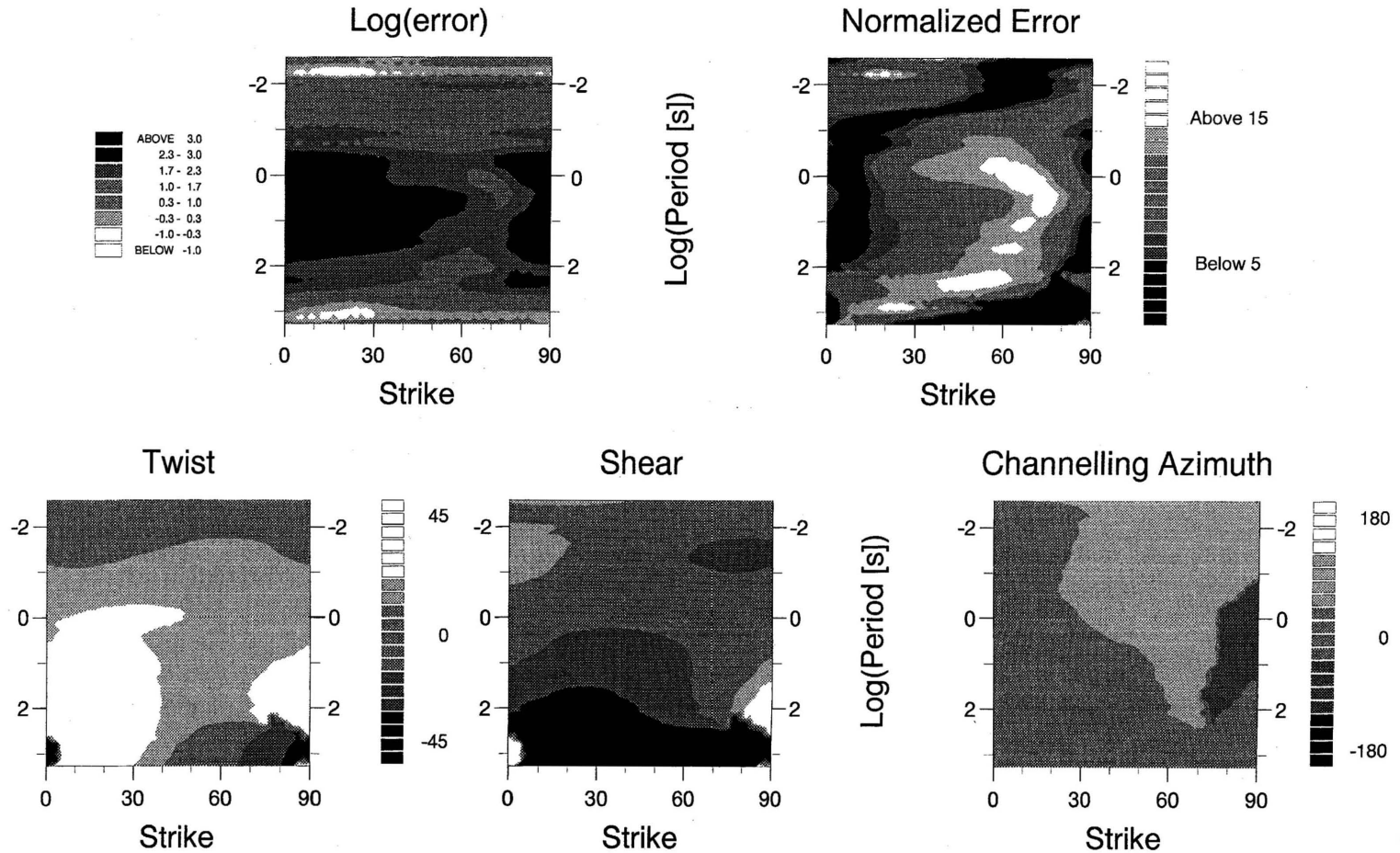
Fig. 3. (b) Grey-scale contour plots of the variation of the decomposition parameters with strike direction from 0° to 90°. The normalized error is a normalized, non-linear, inverted scale (see GKJB); values in excess of 15 ( white ) show strikes which are best-fitting, whereas values less than 5 ( black ) show the worst-fitting strikes.
