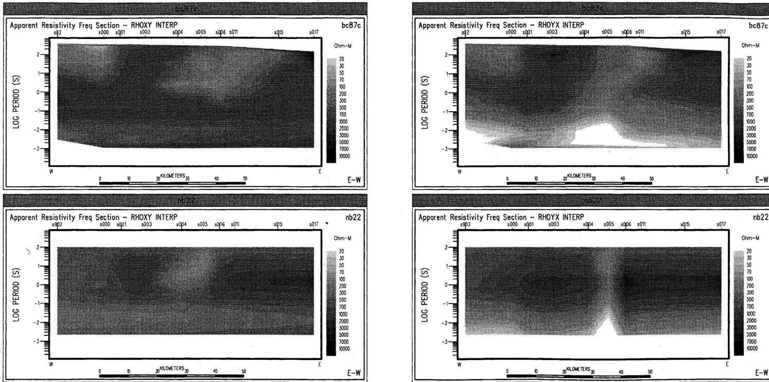
Fig. 15. Comparison of field and model apparent resistivity data for the model illustrated in Fig. 14. The top two pseudosections are the field data, whereas the bottom two are the modelled data. The left column gives the E-polarization responses, whereas the right column gives the B-polarization ones.
