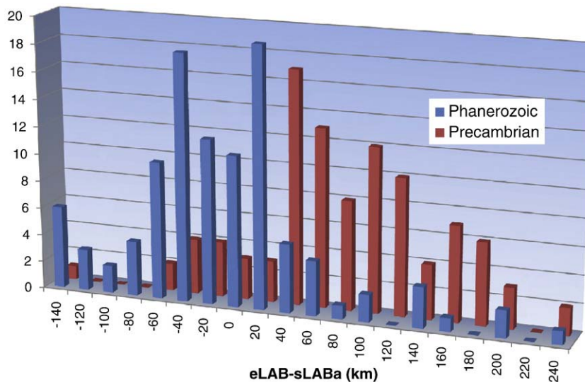
Fig. 16. Histogram of the differences between eLAB and sLABa estimates for Precambrian (red bars) and Phanerozoic (blue bars) Europe.
