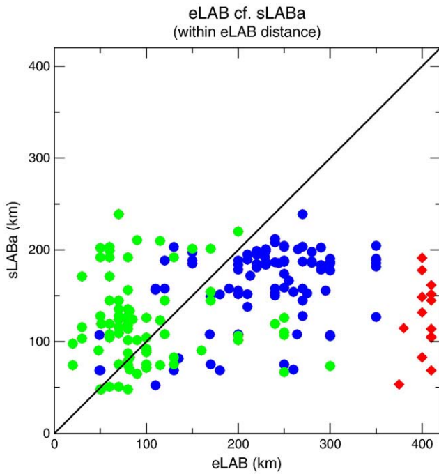
Fig. 14. Cross-plot of raw eLAB against raw sLABa estimates for stations within an eLAB depth of each other. Green points are those from Phanerozoic Europe, blue points are from Precambrian Europe, and the red points are from the locations where the eLAB estimates are ultra-deep just to the north of the TESZ. The solid black line is the 1:1 line that the data should scatter around if there are no bias errors.
